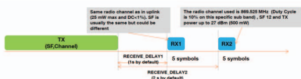
Figure 3 Illustration of used window for DL emissions
