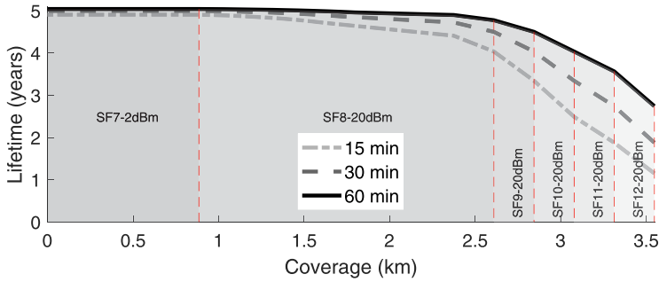
Fig. 18. Setting selections for optimal coverage and lifetime. Exhausting TX Pow before SF would results in a node with better coverage and longer lifetime.
