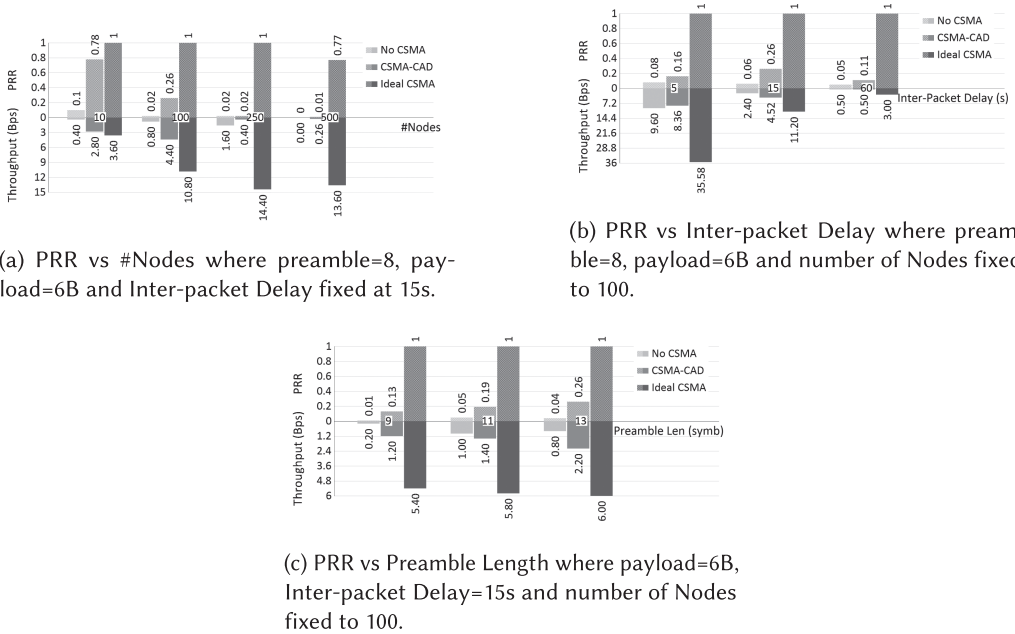
Fig. 27. Simulation of a LoRa network under No-CSMA, CSMA-CAD, and Ideal-CSMA mechanisms. Although Ideal-CSMA mechanism shows promising results, hidden terminal problem and synchronous symbol detection would still cause packet collisions.
