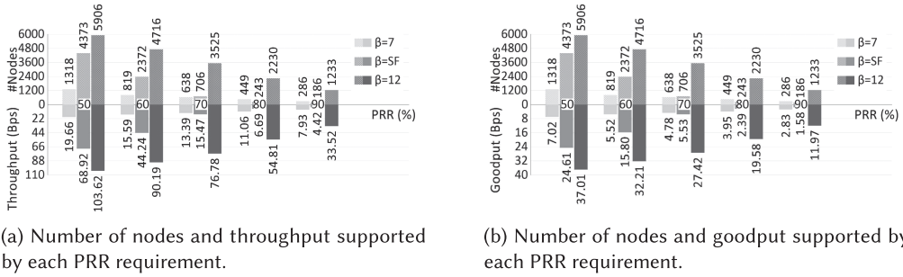
Fig. 22. Comparison of throughput and goodput of a single gateway with LoRaWAN and supported number of nodes for each PRR requirement. Similar to results in Section 3.3, higher number of SF7 packets increases throughput, goodput, and number of supported nodes.
